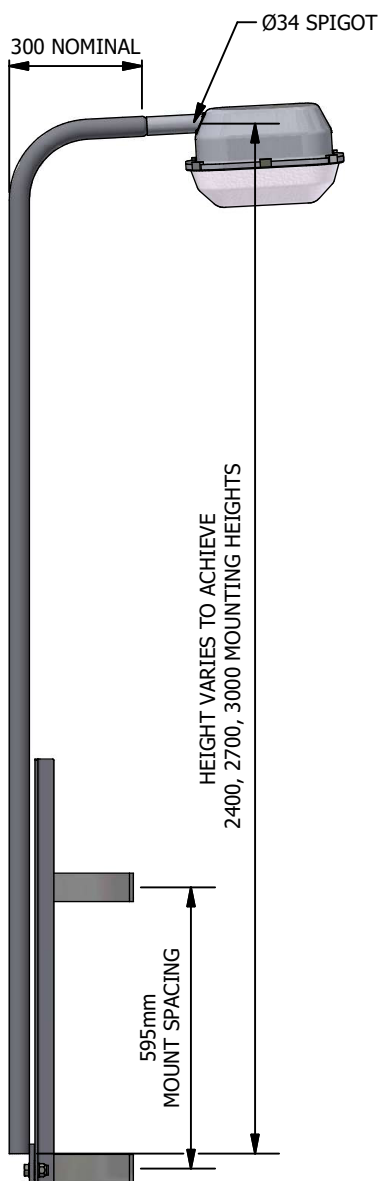
SINGLE HANDRAIL POLE
