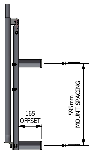
DOUBLE HANDRAIL POLE
